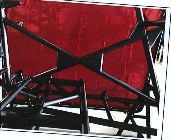
PHOTO 10 ANTI-INTRUSION DOORBAR - DRIVER
