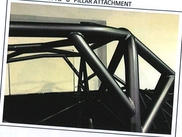
PHOTO 8 MAIN ROLLBAR TO "B" PILLAR ATTACHMENT
