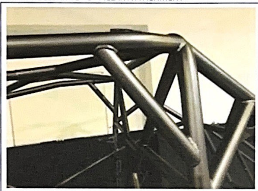
PHOTO 8 MAIN ROLLBAR TO "B" PILLAR ATTACHMENT
