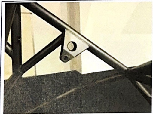
PHOTO 5 REAR BACKSTAY TO BODYSHELL ATTACHMENT
